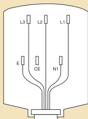
PTO3U (unfused)
