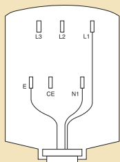
PTO3UR (unfused)
